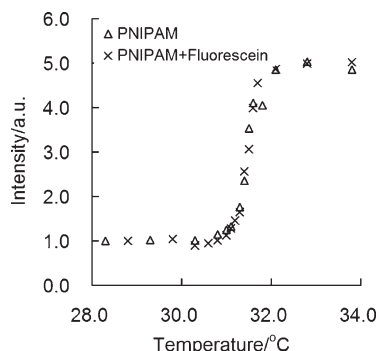
Figure 3. Effect of fluorescein on the phase transition of PNIPAM aqueous solution ( M_w = 2\,400\,000\text{ g mol}^{-1} , C_{\text{PNIPAM}} = 1.14\text{ wt } \% , and C_{\text{fluorescein}} = 10\text{ }\mu\text{M} ) is checked with a dark field microscope, by similarly measuring the scattered light intensity over the phase transition temperature range for the samples with ( \times ) or without ( \Delta ) fluorescein. The fluorescein-containing PNIPAM solution produces negligible difference in the scattering signals and therefore the cloud point, compared to the fluorescein-free solution of the same PNIPAM concentration.
